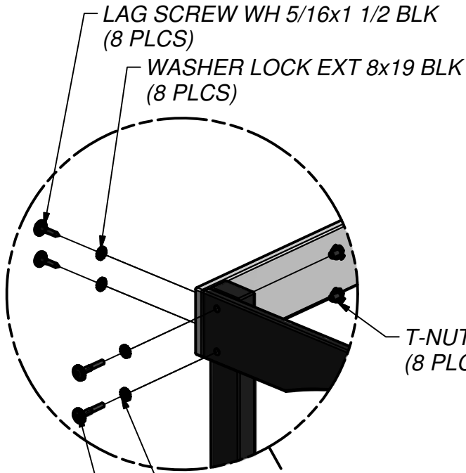
BOLT WH 5/16x2 BLK (8 PLCS) WASHER LOCK EXT 8x19 BLK (8 PLCS)
