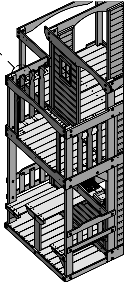
SCREW PFH 8x1 1/8 (32 PLCS)
