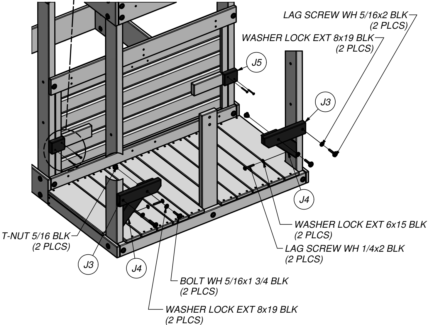
(2) T-NUT 5/16 BLK
